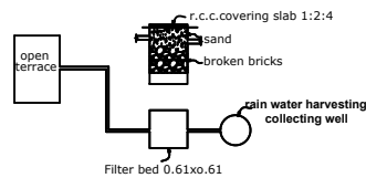
Details of rain water harvesting system
