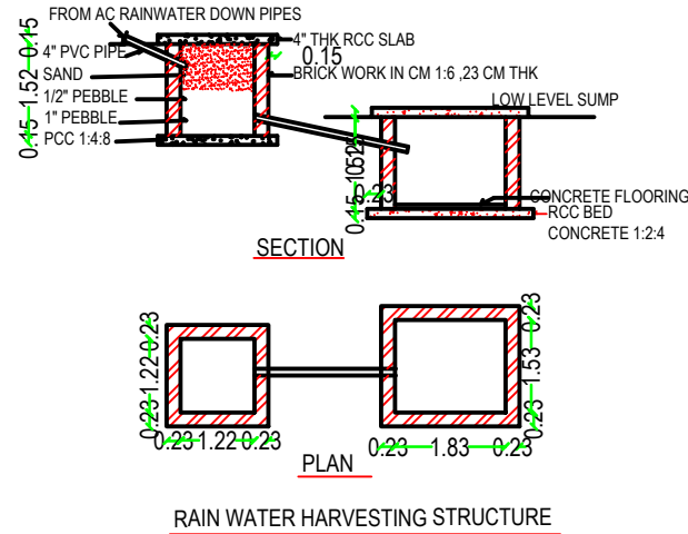
RAIN WATER HARVESTING STRUCTURE
