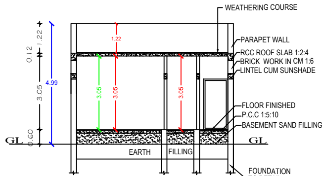
SECTION "J-J"
