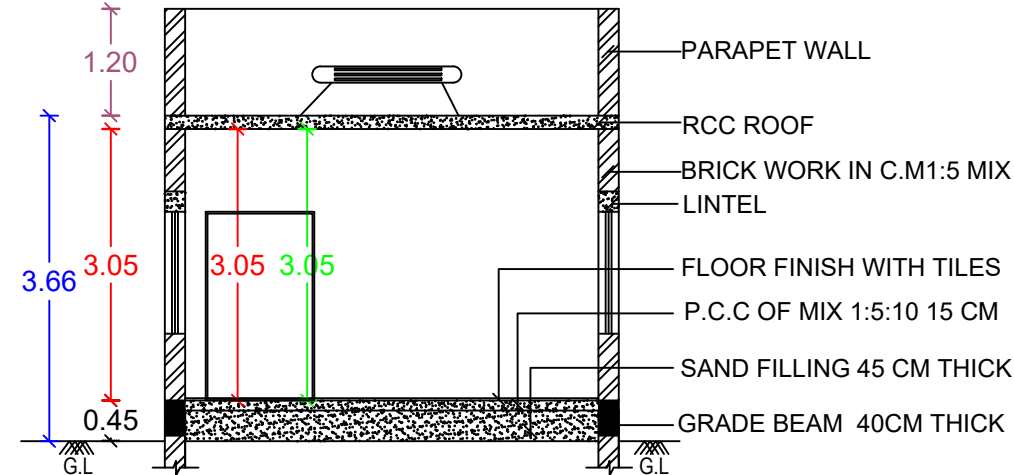
SECTION-AA1
