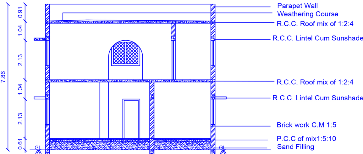
SECTION ON RS
