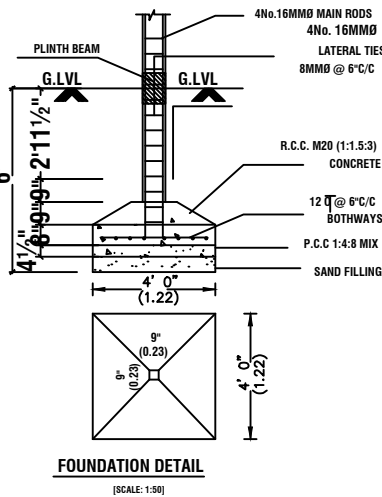
FOUNDATION DETAIL
