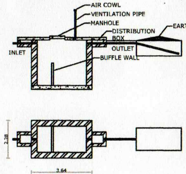
SEPTIC TANK WITH DISPERSION TRENCH
