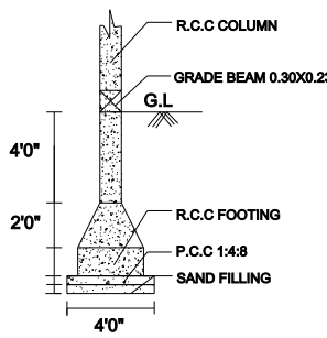
COLOUMN FOUNDATION DETAILS
