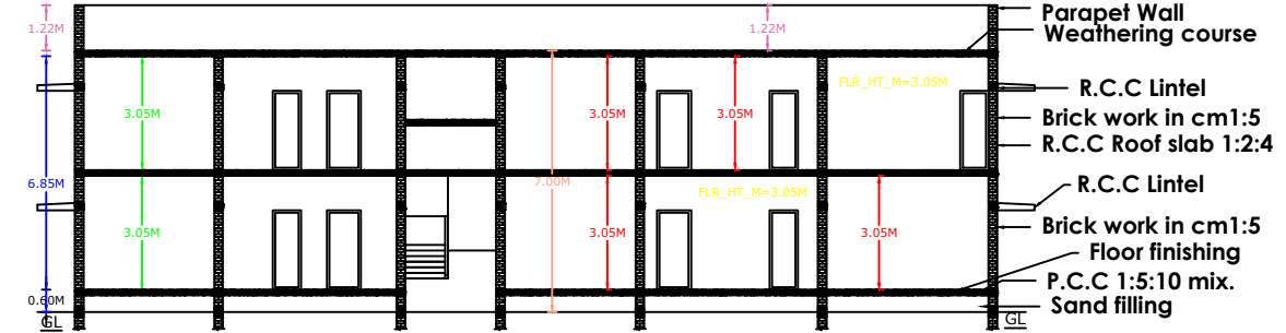
SECTION ON XX
