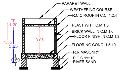
SECTION ON S - S
