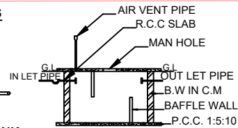
SECTION ON SEPTIC TANK
