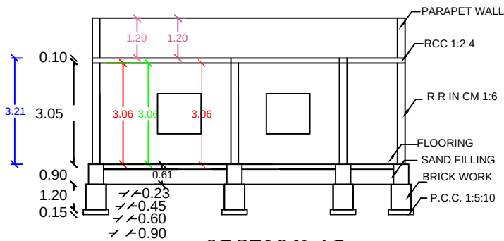
SECTION AB
