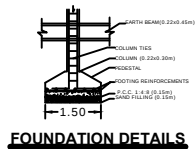
FOUNDATION DETAILS
