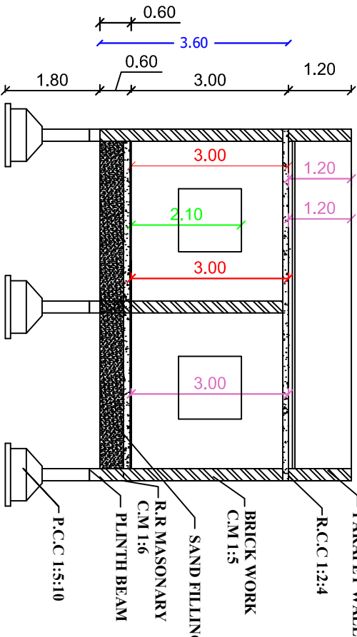
SECTION ON 'AA'
