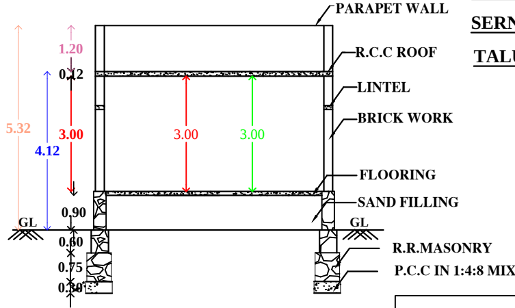
"SECTION "AB"
