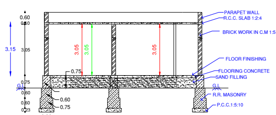
SECTION AB
