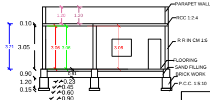
SECTION AB
