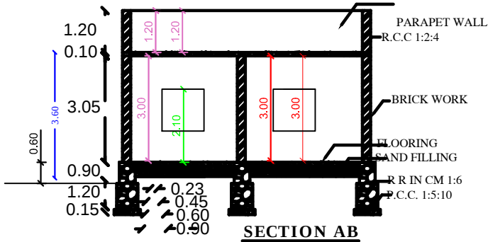
SECTION AB
