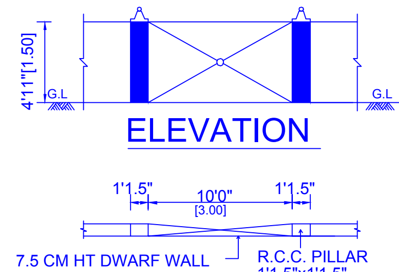
COMPOUND WALL PLAN
