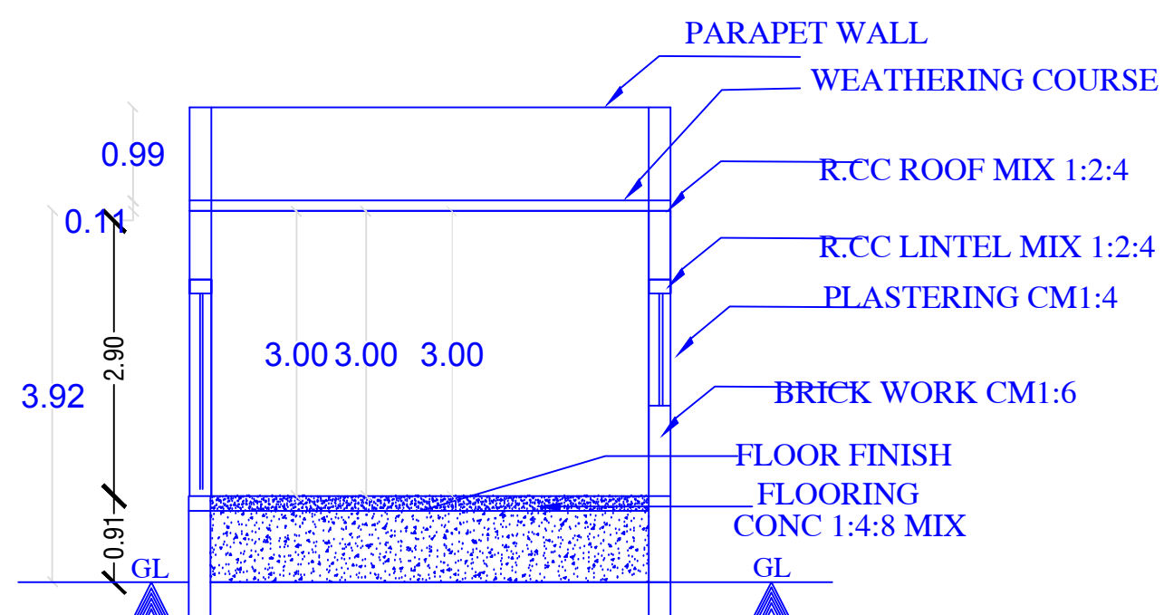
SECTION : "A-A"
