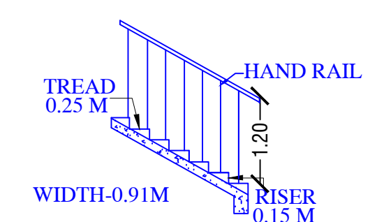
STAIRCASE DETAILS
