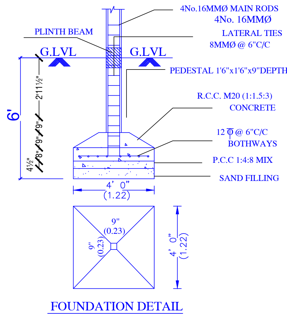
FOUNDATION DETAIL
