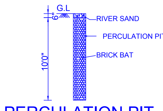
PERCOLATION PIT
