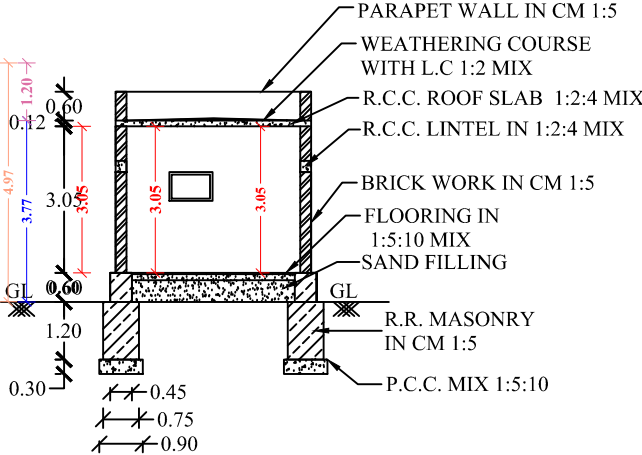
SECTION OF "AB"
