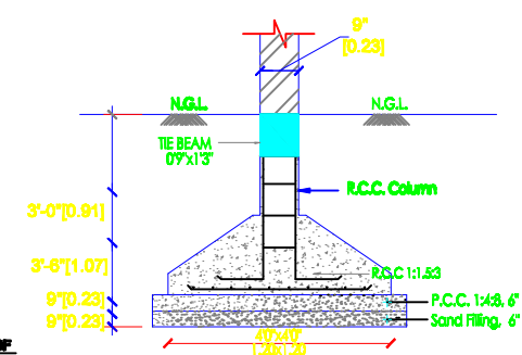
FOUNDATION DETAIL
