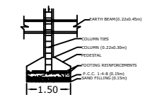
FOUNDATION DETAILS
