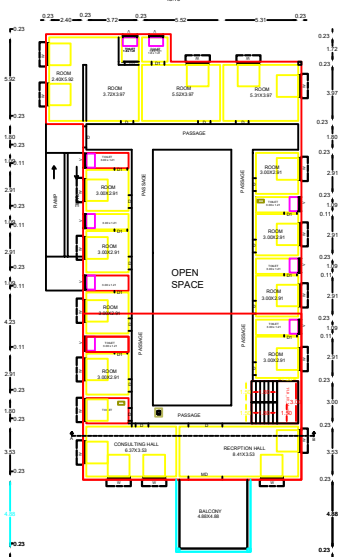
EXT FIRST FLOOR COMMERCIAL PLAN
