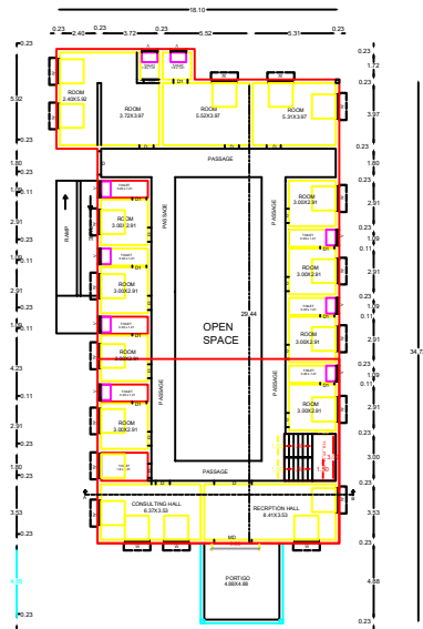
EXT GROUND FLOOR COMMERCIAL PLAN
