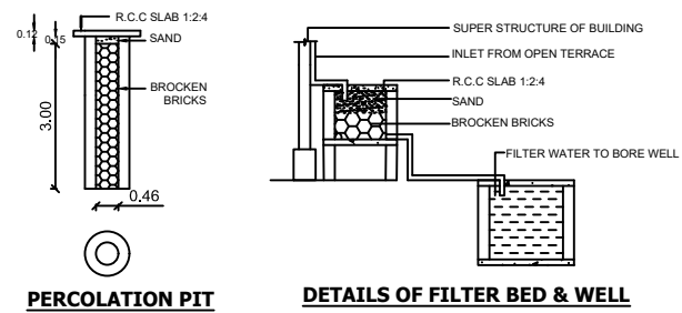
PERCOLATION PIT
