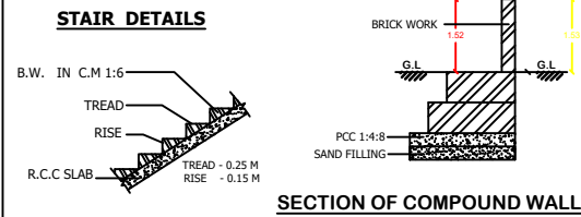
SECTION OF COMPOUND WALL
