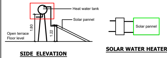
SIDE ELEVATION
