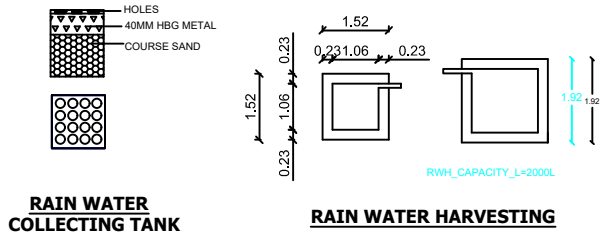
RAIN WATER HARVESTING
