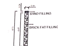
DETAILS OF PERCULATION PIT
