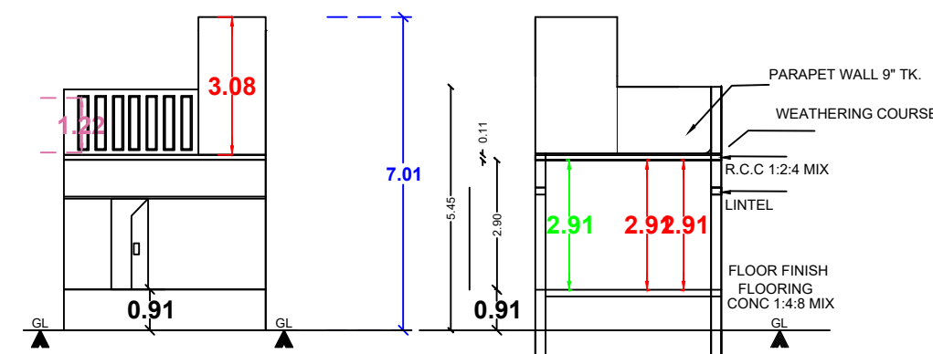
FRONT ELEVATION SECTION : "A-A"
