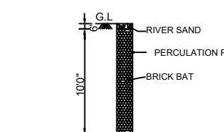
PERCOLATION PIT
