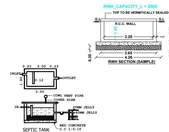
SEPTIC TANK
