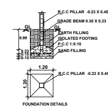
FOUNDATION DETAILS
