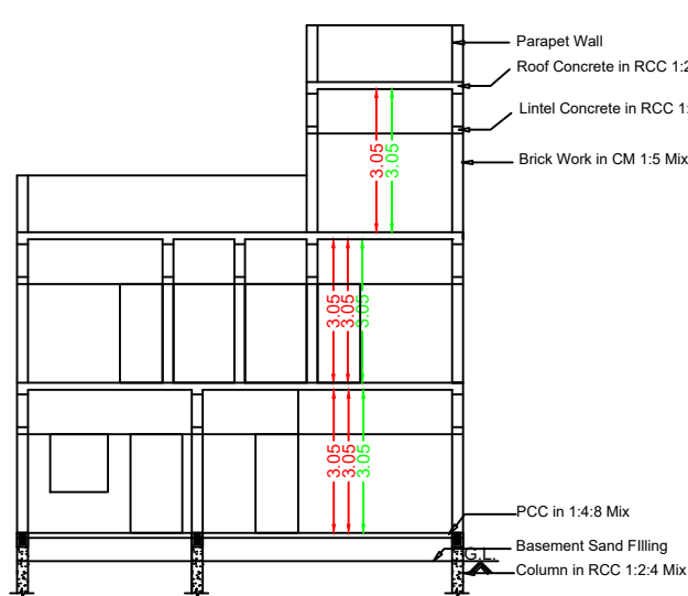
Section RR
