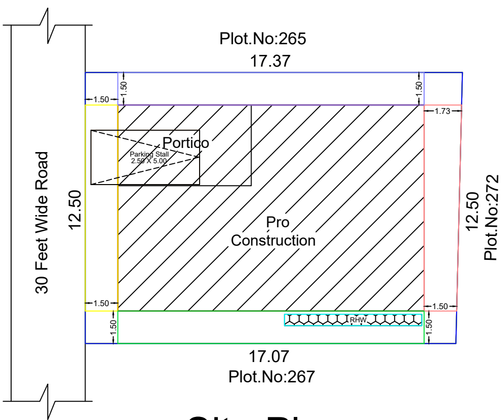
Site Plan
