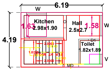
FLOOR - PLAN
