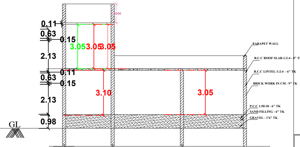
SECTION
