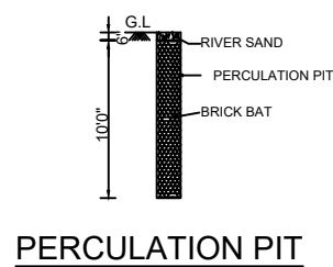
PERCULATION PIT
