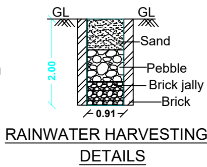
RAINWATER HARVESTING DETAILS
