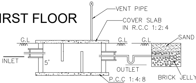
SECTION-AB
