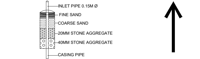
DETAILS OF RAIN WATER HARVESTING STRUCTURES (NOT to SCALE)
