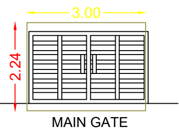
MAIN GATE
