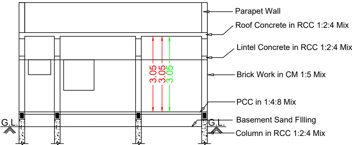
Section RR
