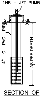
SECTION OF
