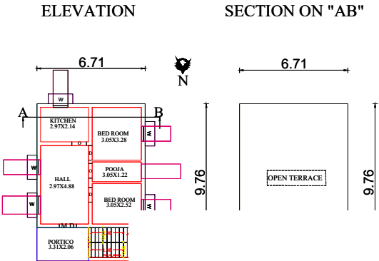
PROPOSED GRO FLOOR PLA
