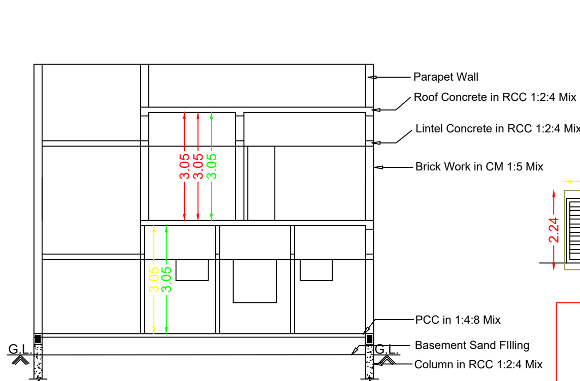
Section RR
