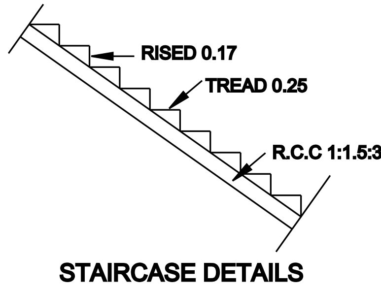
STAIRCASE DETAILS
