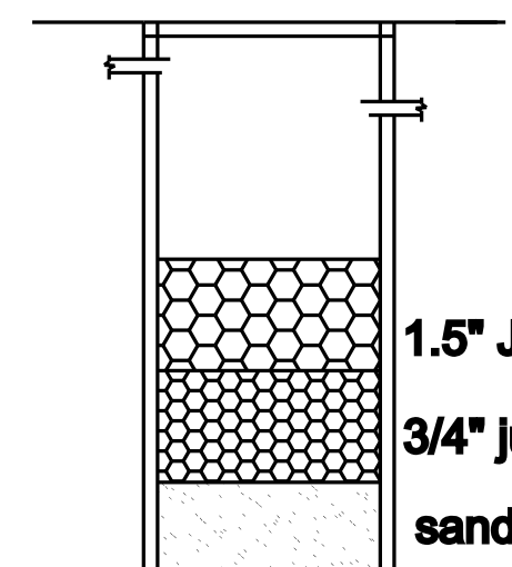
RAIN WATER HARVESTING TANK
