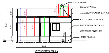
CUT SECTION ON AA
