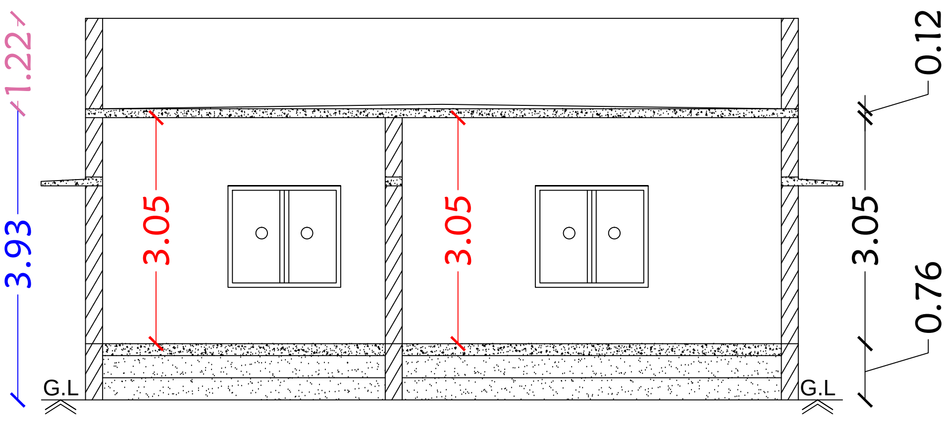
Section on-"AA"
