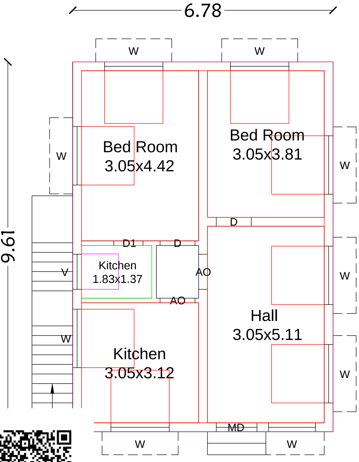
Ground Floor
