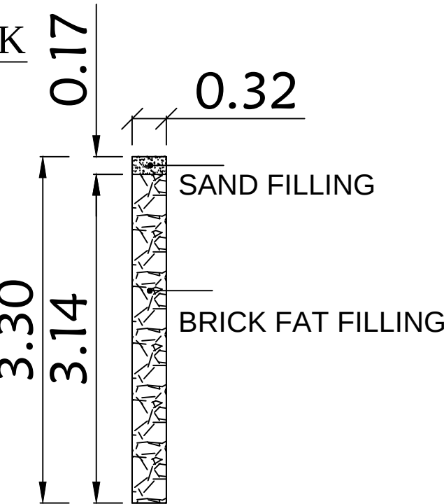
DETAILS OF PERCULATION PIT
