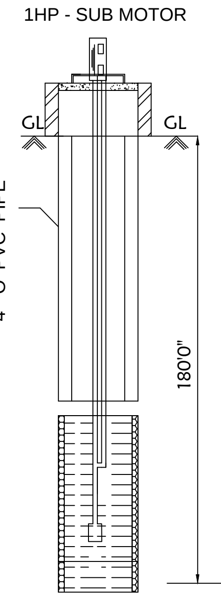
Bore Well Details
