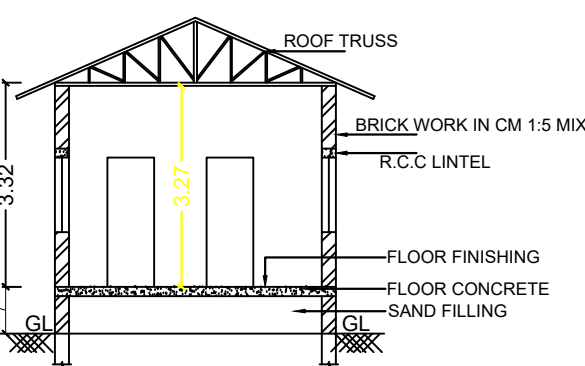
SECTION AT A1-A1
