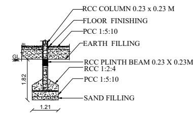
FOUNDATION DETAILS
