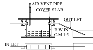
DETAILS OF SEPTIC TANK & D-TRENCH
