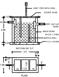
SEPTIC TANK DETAILS (NOT TO SCALE)
