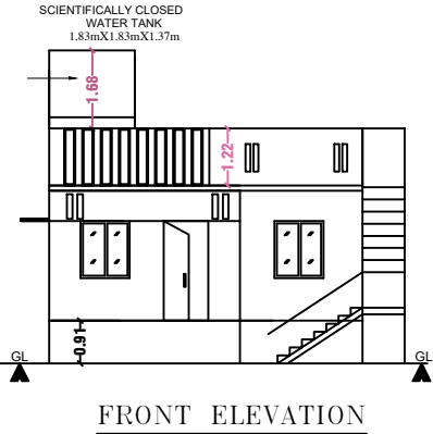
FRONT ELEVATION
