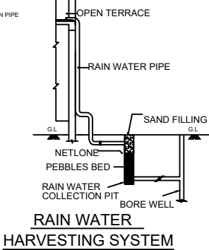
SECTION - CC
