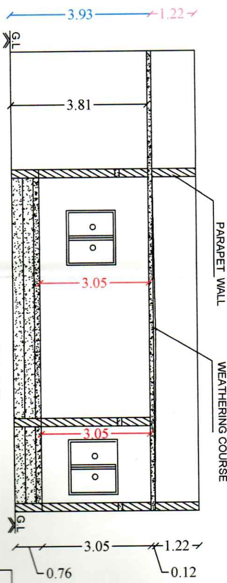
Section on-"AA"
