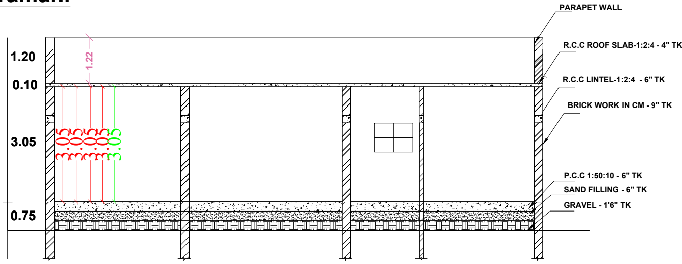
SECTION AB
