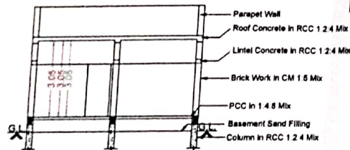
Section RR
