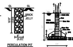
FOUNDATION DETAILS SCALE : 1:50
