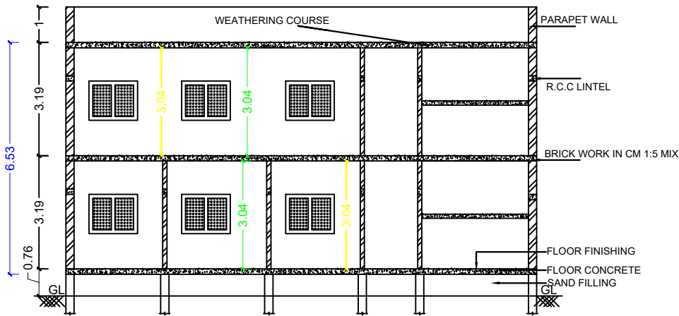
SECTION AT A1-A1
