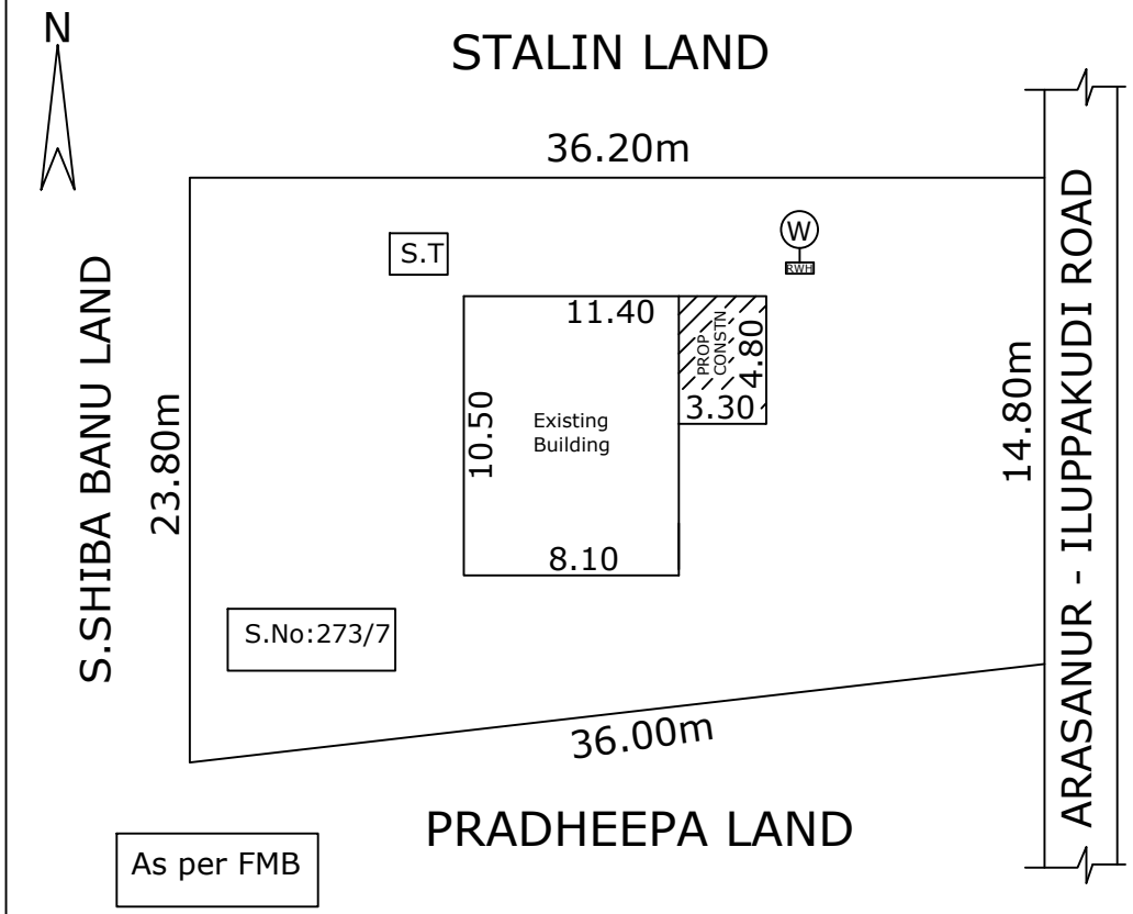
SITE PLAN
