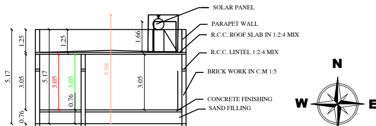
CUT SECTION ON AA
