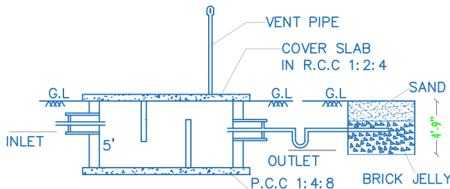
SECTION-AB
