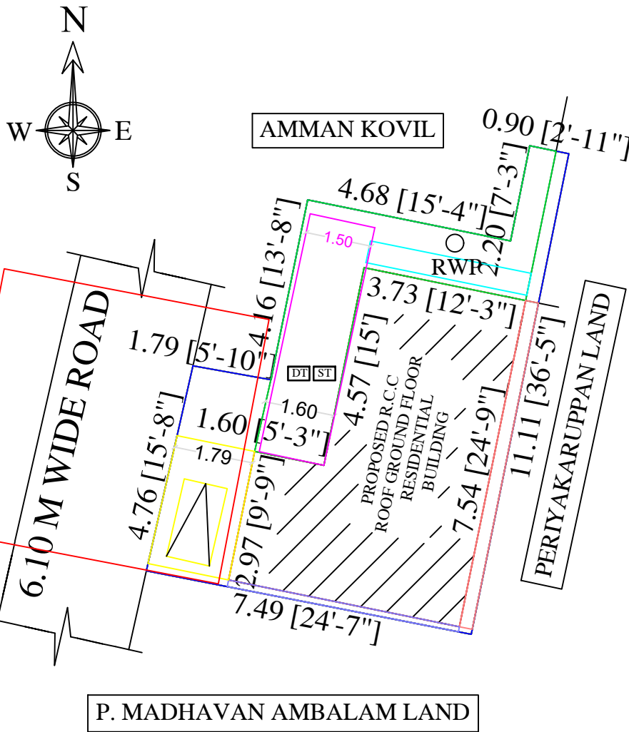
SITE PLAN
