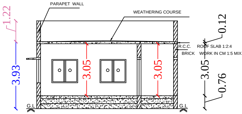
Section on-"AA"
